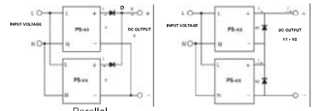
Parallel (D: ORing diode)
